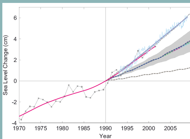
Figure 1: Change in sea level from 1970 to 2008, relative to the sea level at 1990. The solid lines are based on observations smoothed to remove the effects of interannual variability (light lines connect data points). Data in most recent years are obtained via satellite-based sensors. The envelope of IPCC projections is shown for comparison; this includes the broken lines as individual projections and the shading as the uncertainty around the projections.
